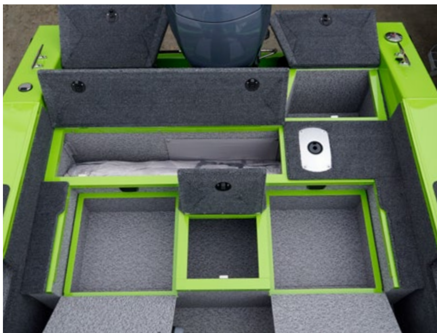
Configuration JS has a large number of stern deck lockers with a total volume of 290 liters.
